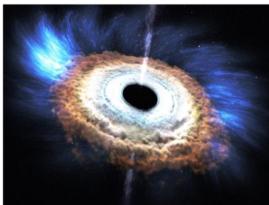
Fig. 8. Black hole in singularity condition.
