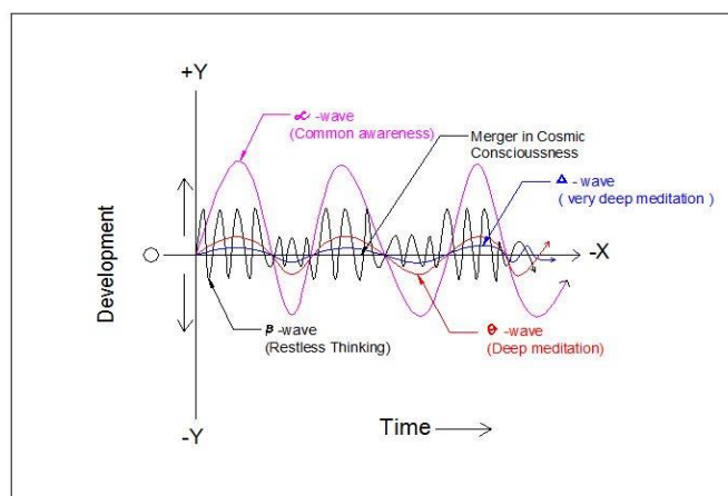
Fig. 10. Alpha, Beta, Delta, and Theta Waves.
