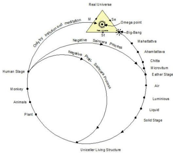
Fig. 5. Sristi-Chakra with Big-bang.
