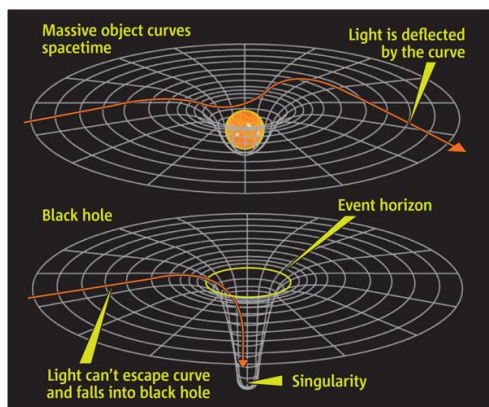
Fig. 9. Singularity condition in Black-hole.
