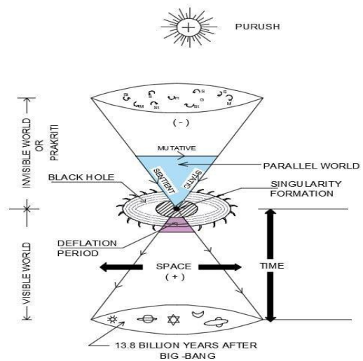
Figure :7 CREATION OF UNIVERSE FROM BLACK HOLE OR SAGUNBRAMAN
