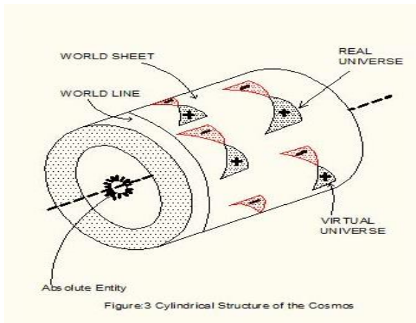
Fig. 2 Cylindrical Structure of Cosmos.
