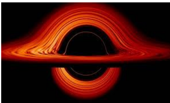
Fig. 3 Prakriti's three forces swirling around omega point in the Black hole.
