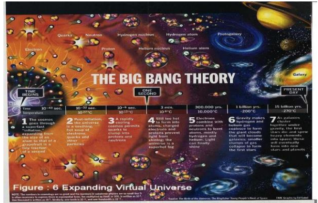
Fig. 6. Expanding Virtual Universe. Source: The birth of the Universe, The Kingfisher Young People’s Book of Space
